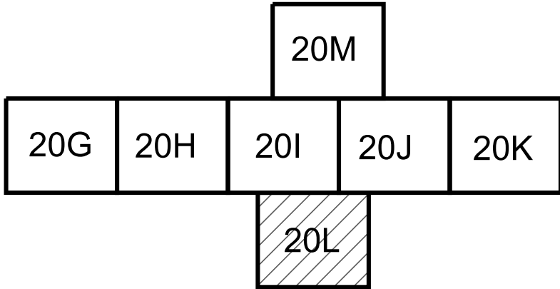
Keymap
